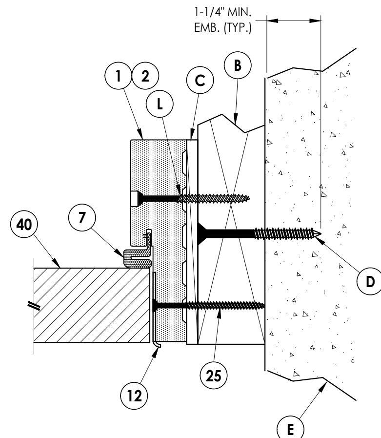
2 HORIZONTAL CROSS SECTION 4 Outwing Shown (Inswing Similar) Shown w/ 2X Buck
